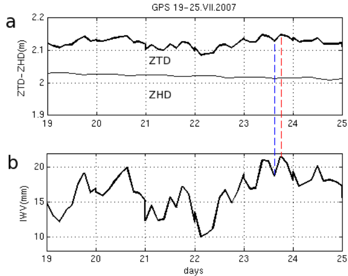
Figure 3. Temporal variation of: a)ZTD and ZHD and b)IWV at GNSS SOFI station during 19-25 July 2007 heat wave.
