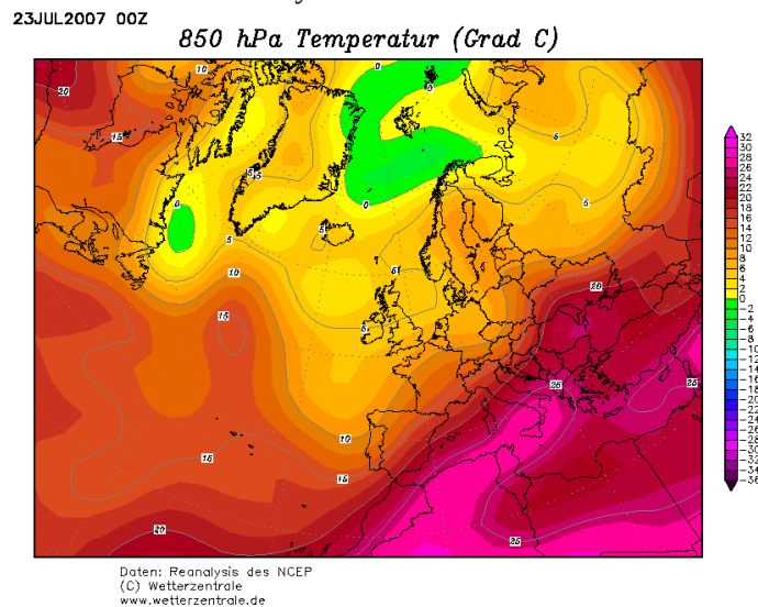
Figure 4. Temperature at 850hPa (1.5 km msl.) on 23 July 2007 00UTC.
