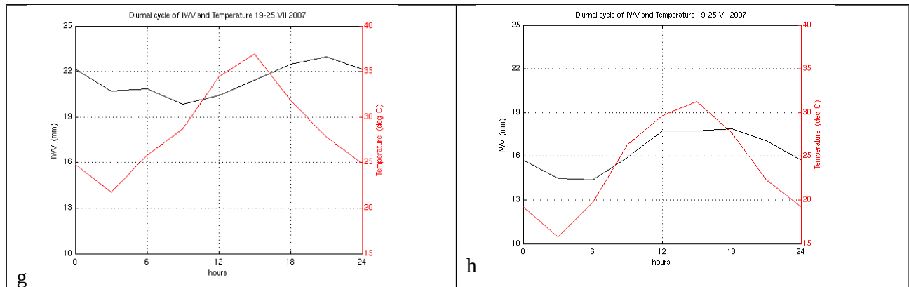
Figure 5. Diurnal cycle of IWV in mm (black line) and temperature in °C (red line) for : a) Bucharest, Romania; b) Craiova, Romania; c) Constanta, Romania; d) Varna, Bulgaria; e) Athens, Greece; f) Dubrovnik, Croatia; g) Thessaloniki, Greece and h) Sofia, Bulgaria.
